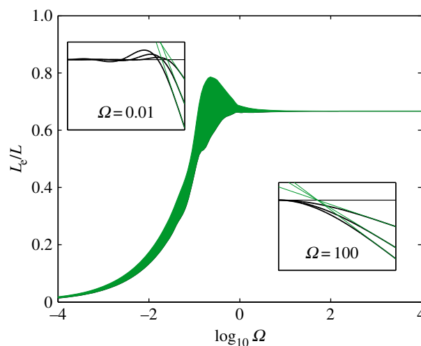
Figure 11. Effective length of a clamped beam as a function of the dimensionless stiffness \Omega . The thickness of the line is proportional to the standard deviation of L_e(\tau) and reveals the extent to which it is time independent and well defined. Insets represent the beam deformation over time for two different values of \Omega . The effective length is defined as the distance between the tip of the beam and the intersection of green (light grey) lines with the horizontal. (Online version in colour.)
