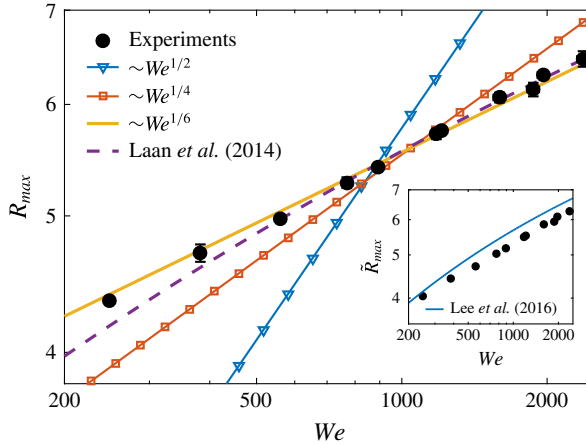
FIGURE 5. (Colour online) Comparison of our measured isolated drop R_{max} = r_{max}/r_1 as a function of impact Weber number We (black dots) with literature predictions summarized in table 1. Our data, obtained with the conditions summarized in table 5, are best captured by R_{max} = 0.61(We/Oh)^{1/6} from Scheller & Bousfield (1995). Here, the Weber number We = \rho u_1^2 (2r_1)/\sigma and the Ohnesorge number Oh = \mu/\sqrt{\rho\sigma(2r_1)} .
